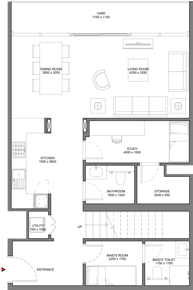
LOWER LEVEL
