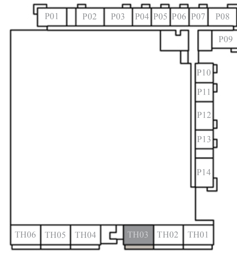
PODIUM FLOOR
