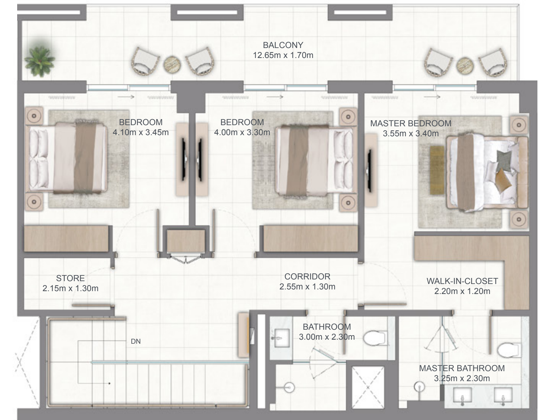
UPPER FLOOR
