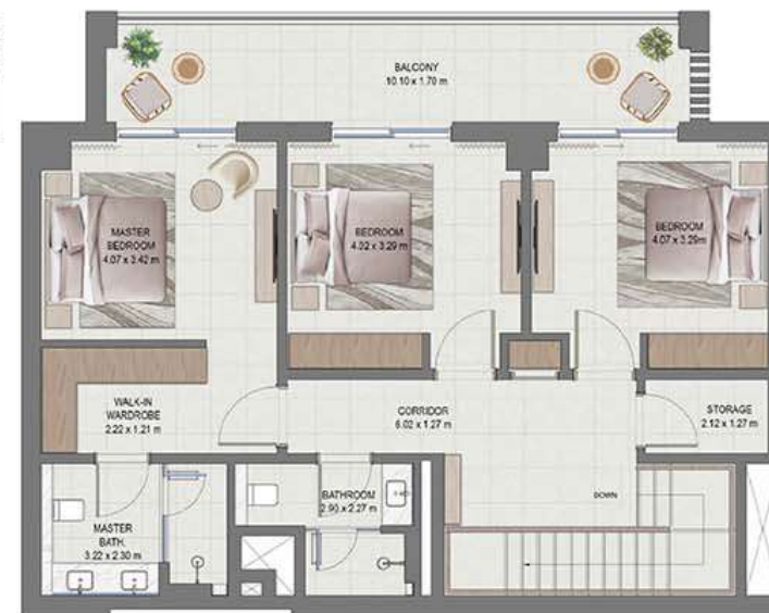
UPPER FLOOR
