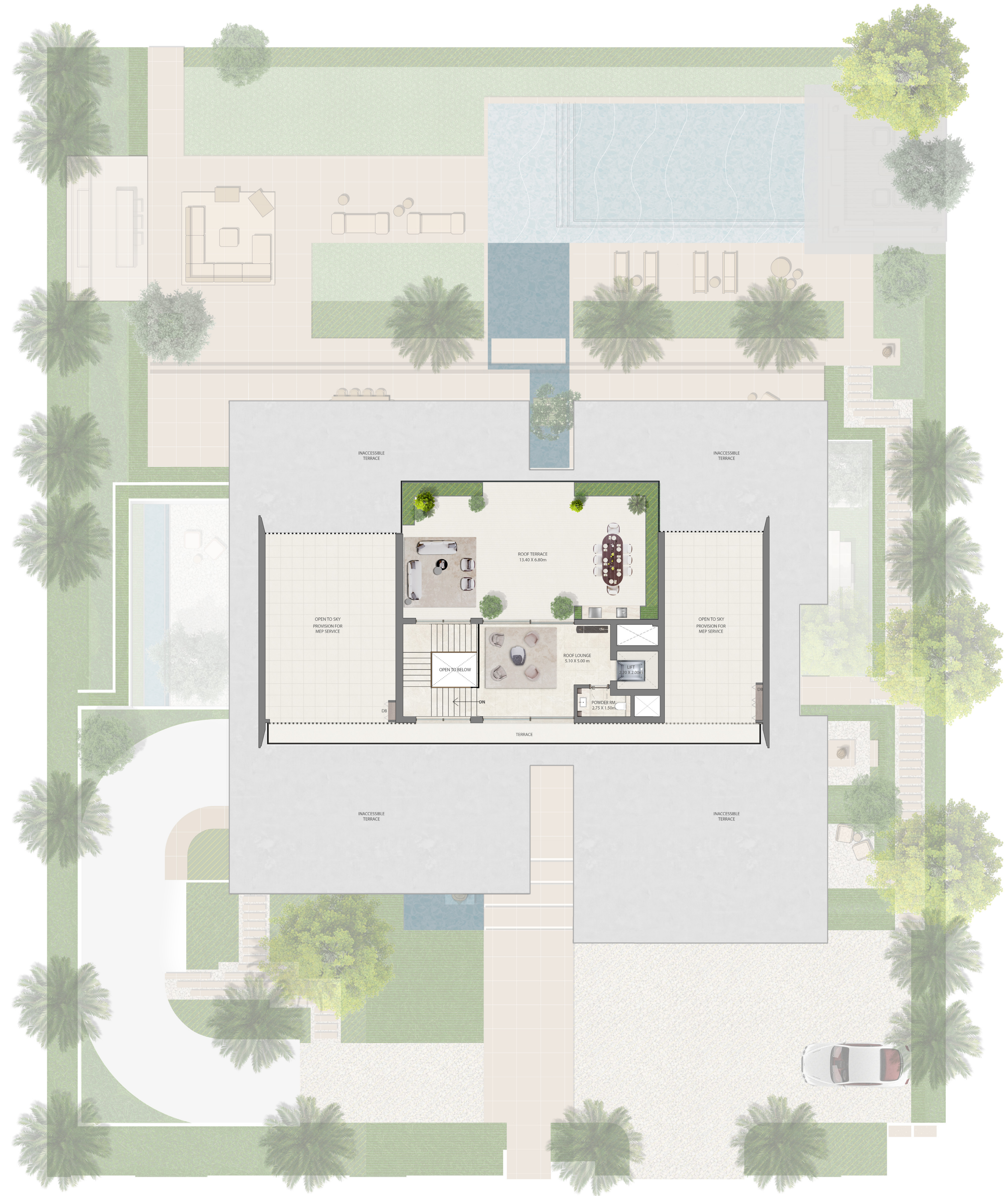
ROOF FLOOR
