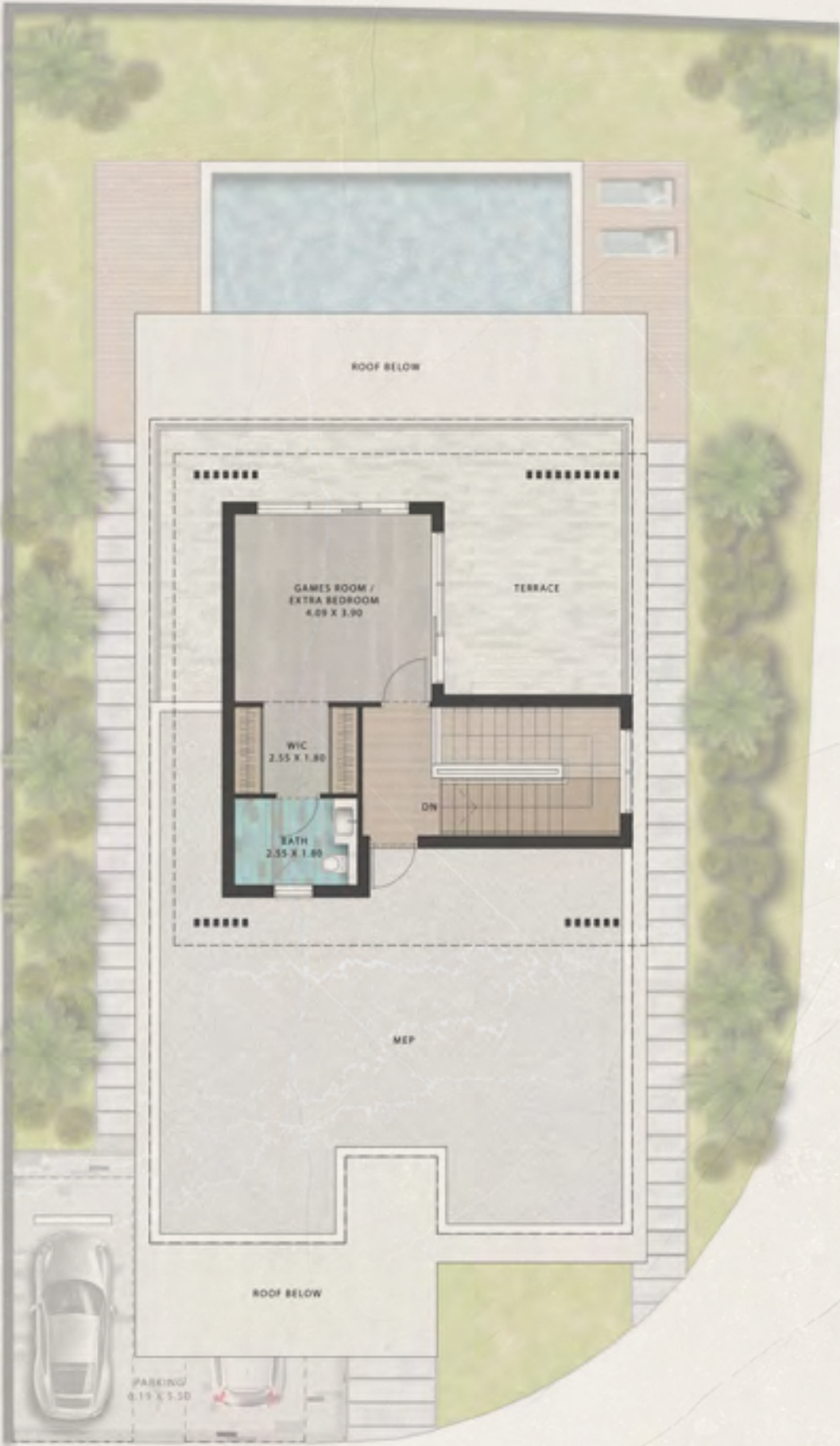
ROOF FLOOR
