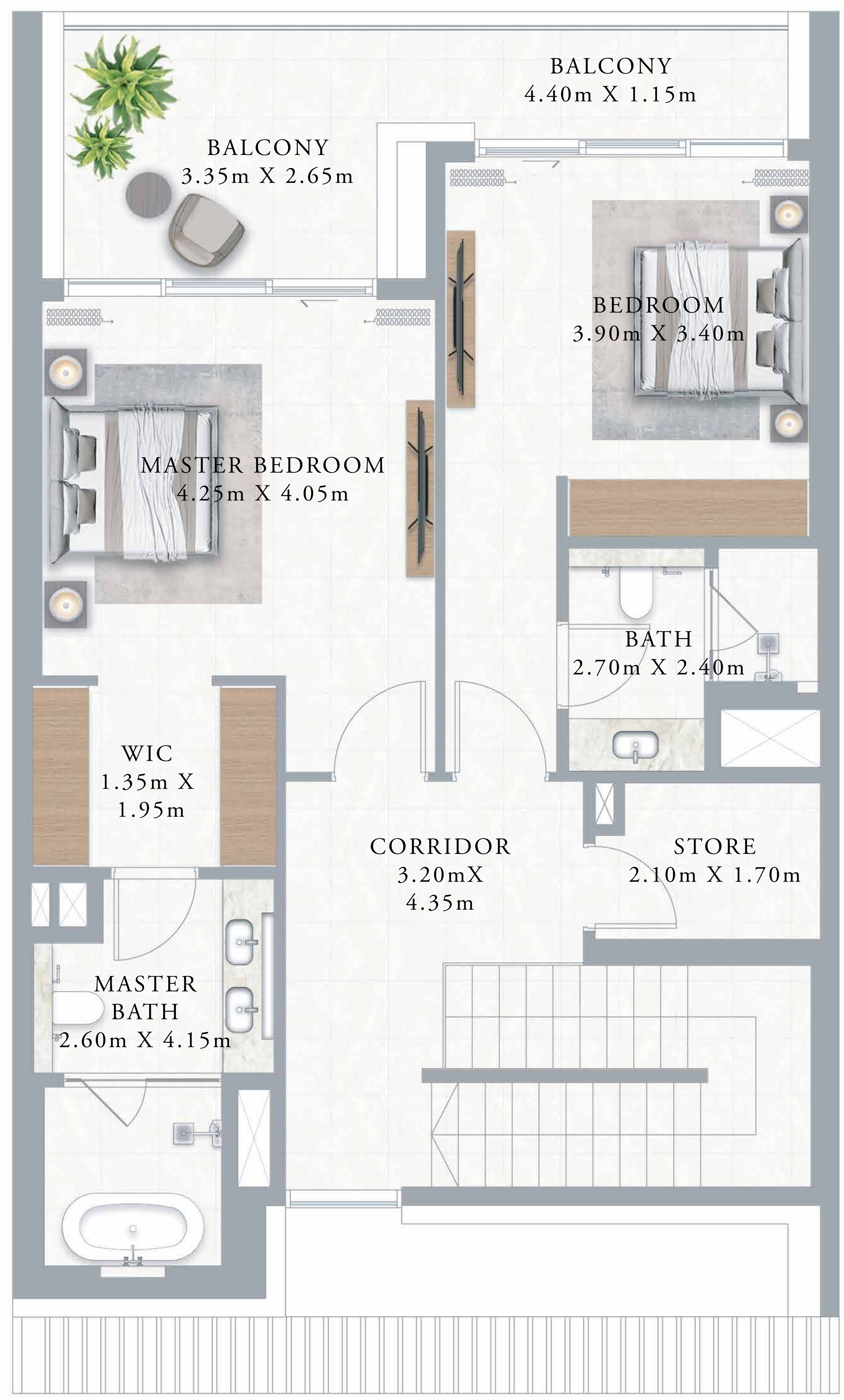
UPPER LEVEL
