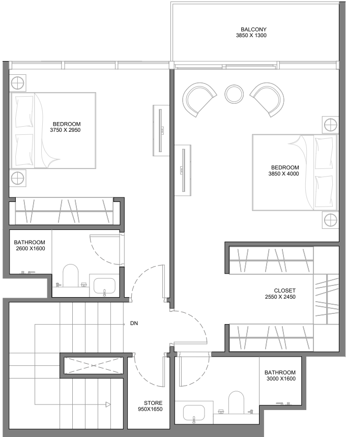
UPPER LEVEL
